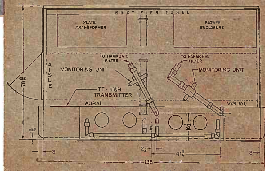
Typical floor plan arrangement for the TT-11AH transmitter, showing rectifier enclosure placed immediately behind the front line of the cabinets. (Rectifier may be remotely located if desired.) The wide aisle provides accessibility to rear components.
